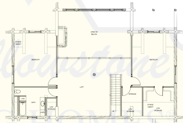
SECOND LEVEL
