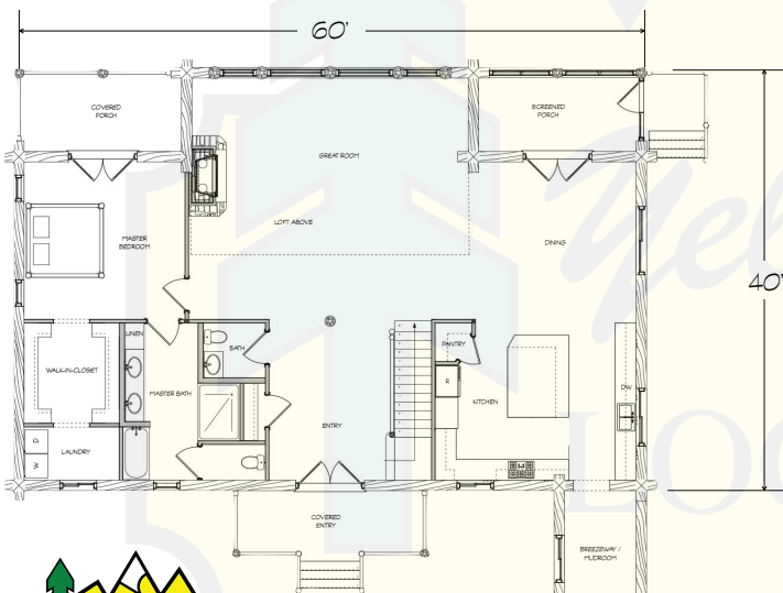
MAIN LEVEL
