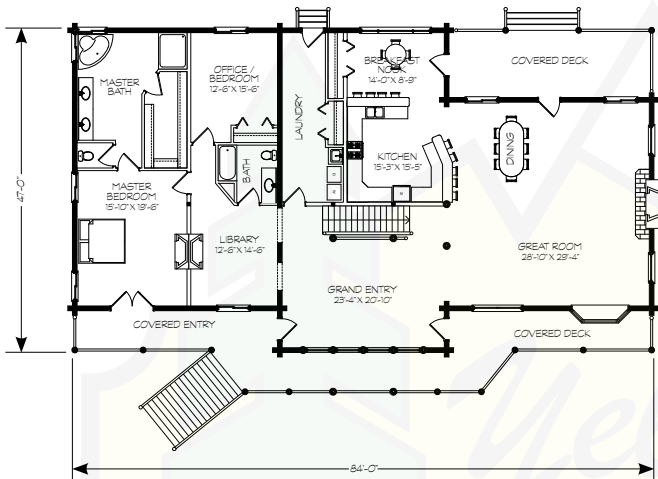
MAIN LEVEL
