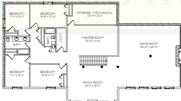
BASEMENT
